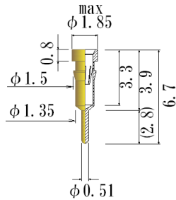
Acceptable plug: \phi 0.60 \sim \phi 0.40 J0010-L-GG
